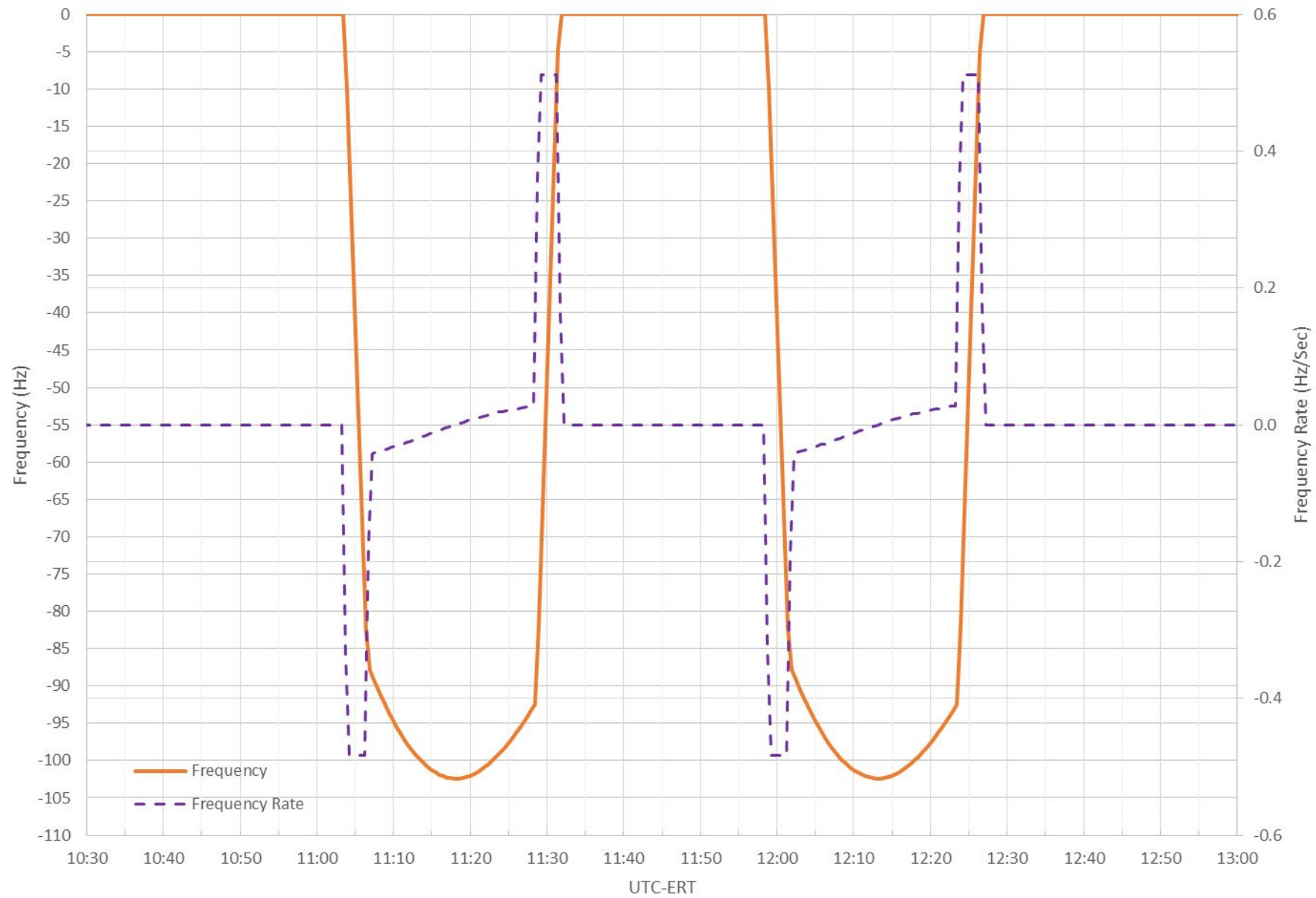
2016/240 DSS-35 X-Band Downlink Frequency Difference due to Imposed Doppler Uncertainty
