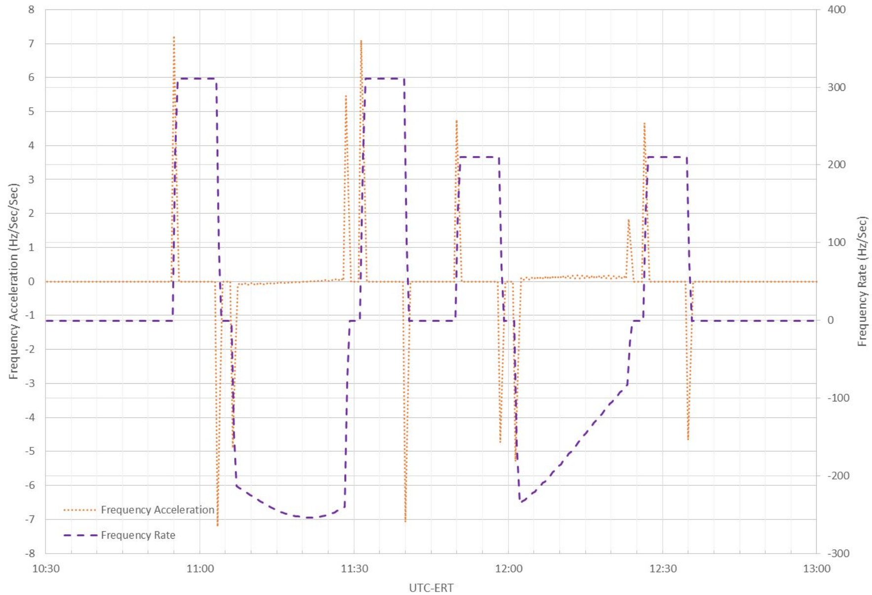
2016/240 DSS-35 2-Way X-Band Downlink Frequency Acceleration & Rate
