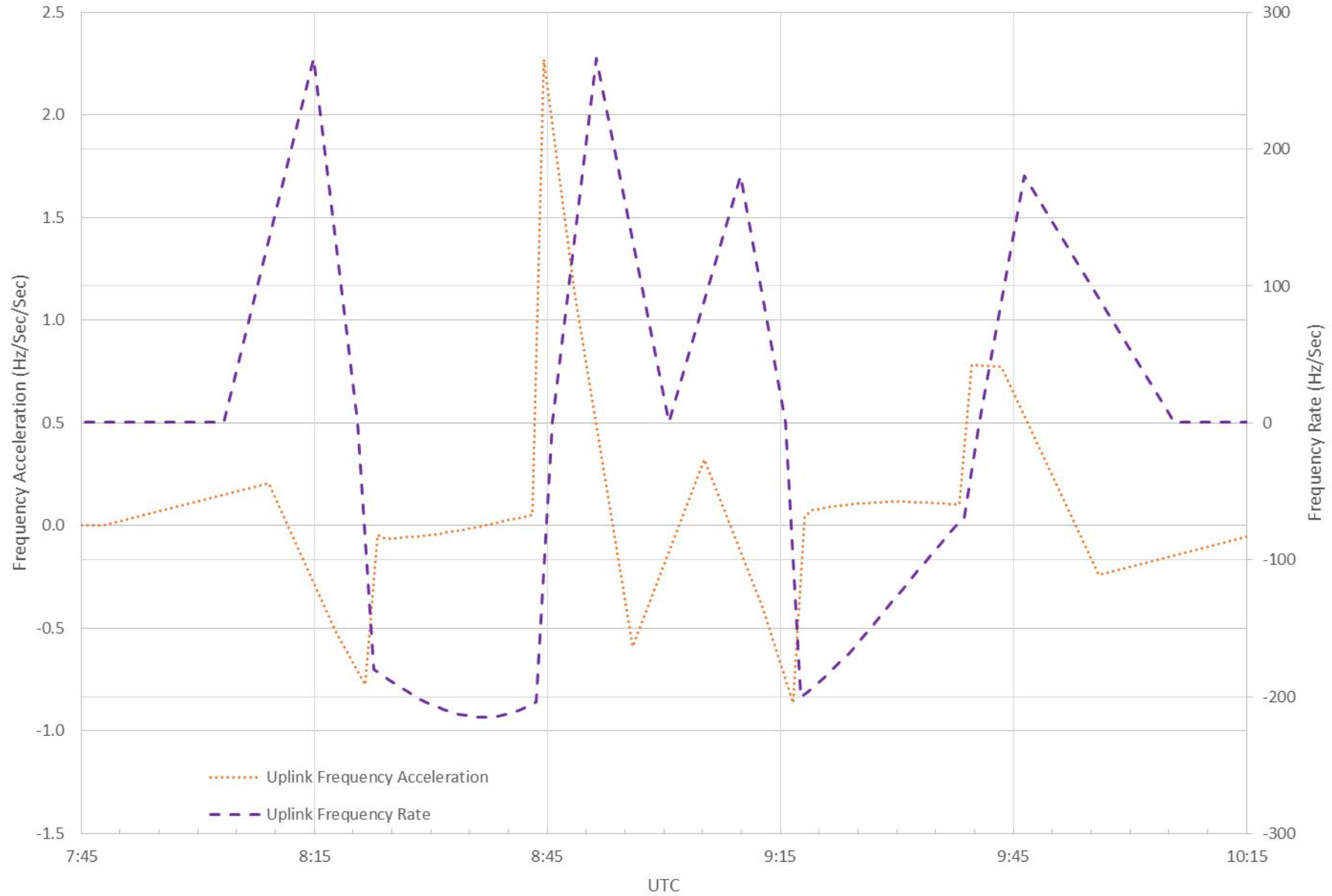
2016/240 DSS-35 Modified Uplink Ramp Acceleration & Rate
