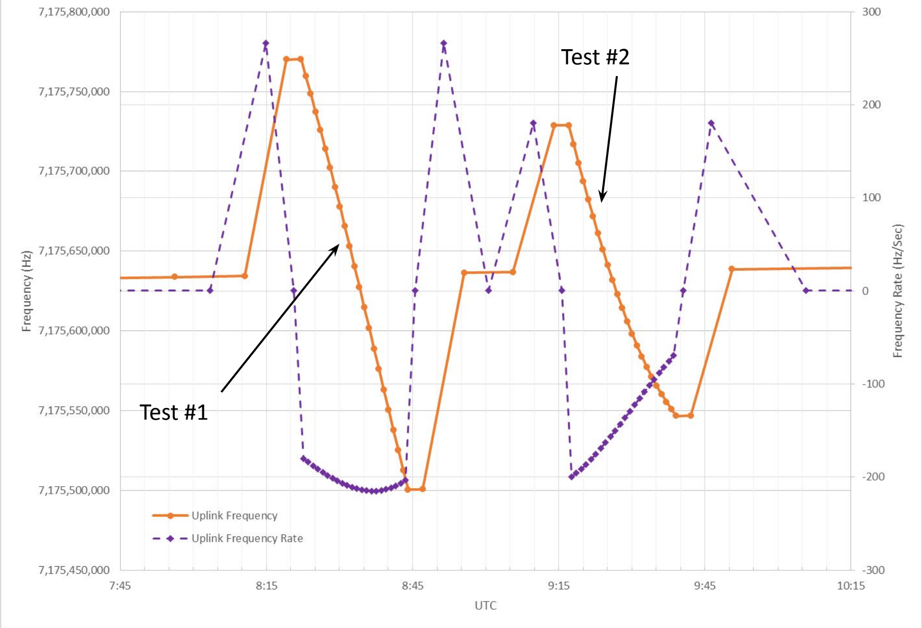
2016/240 DSS-35 Modified Uplink Ramp Frequency & Rate
