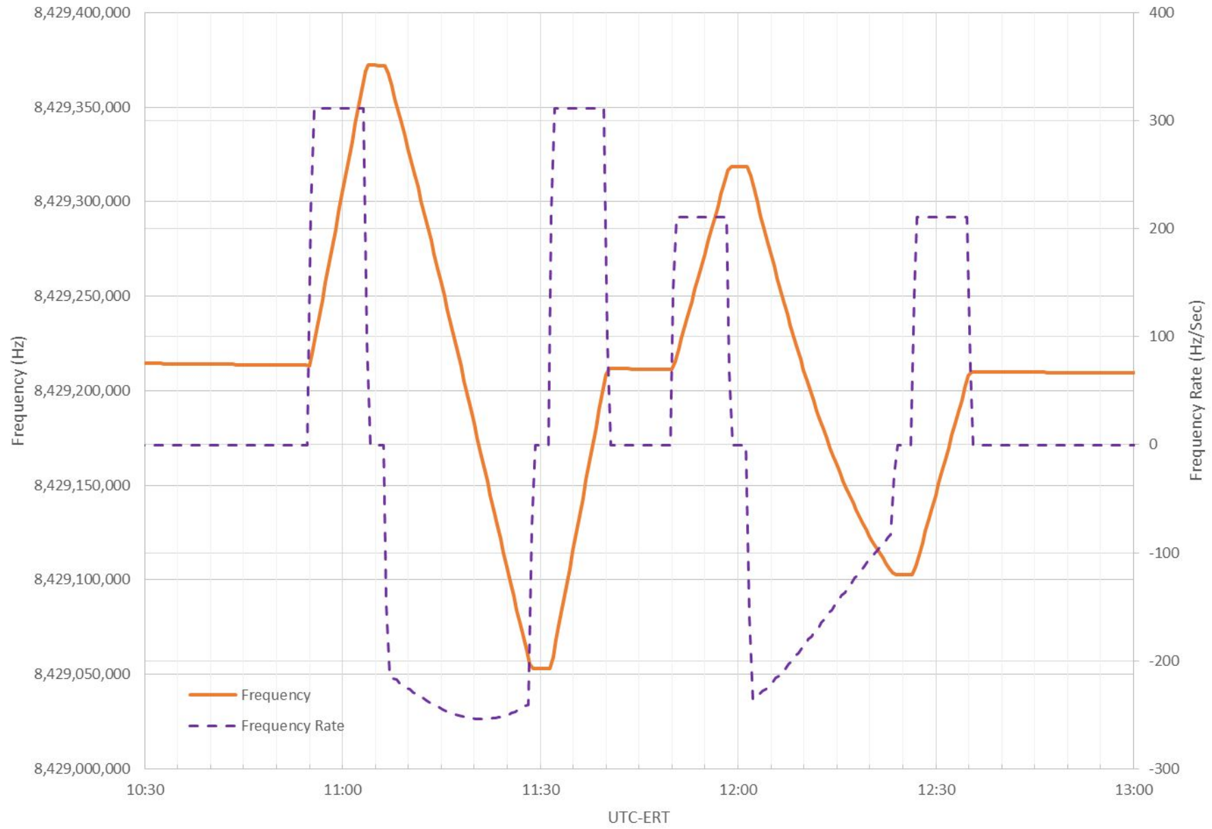
2016/240 DSS-35 2-Way X-Band Downlink Frequency & Rate
