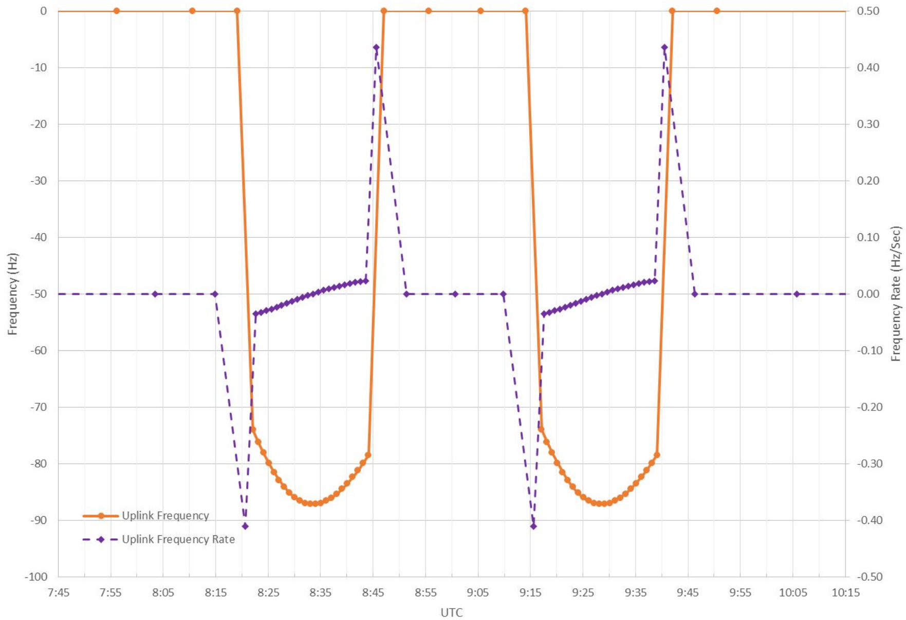
2016/240 DSS-35 Uplink Ramp Difference due to Imposed Uncertainty
