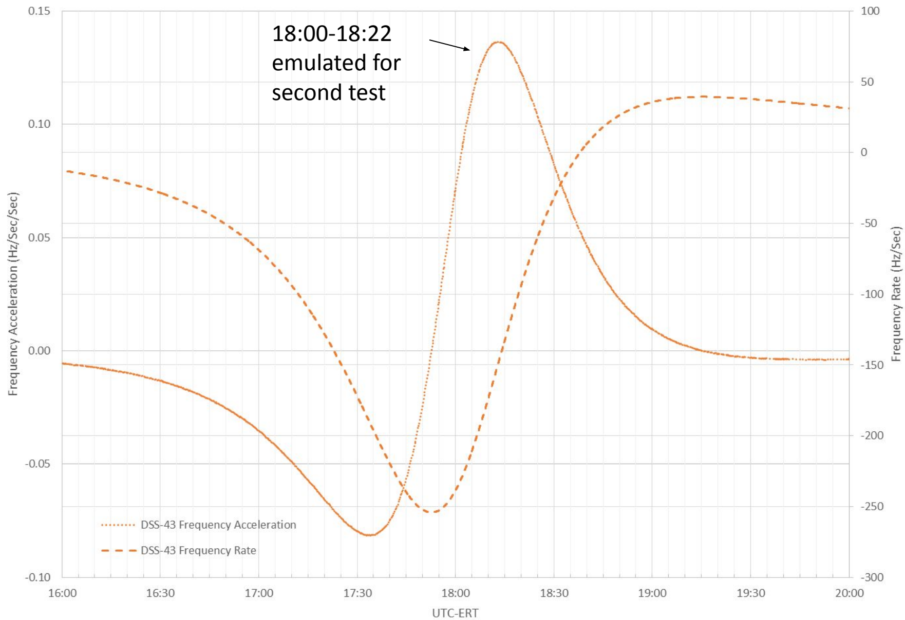
2017/135 18:02 Closest Approach (1-Way X-Band Downlink) Acceleration & Rate
