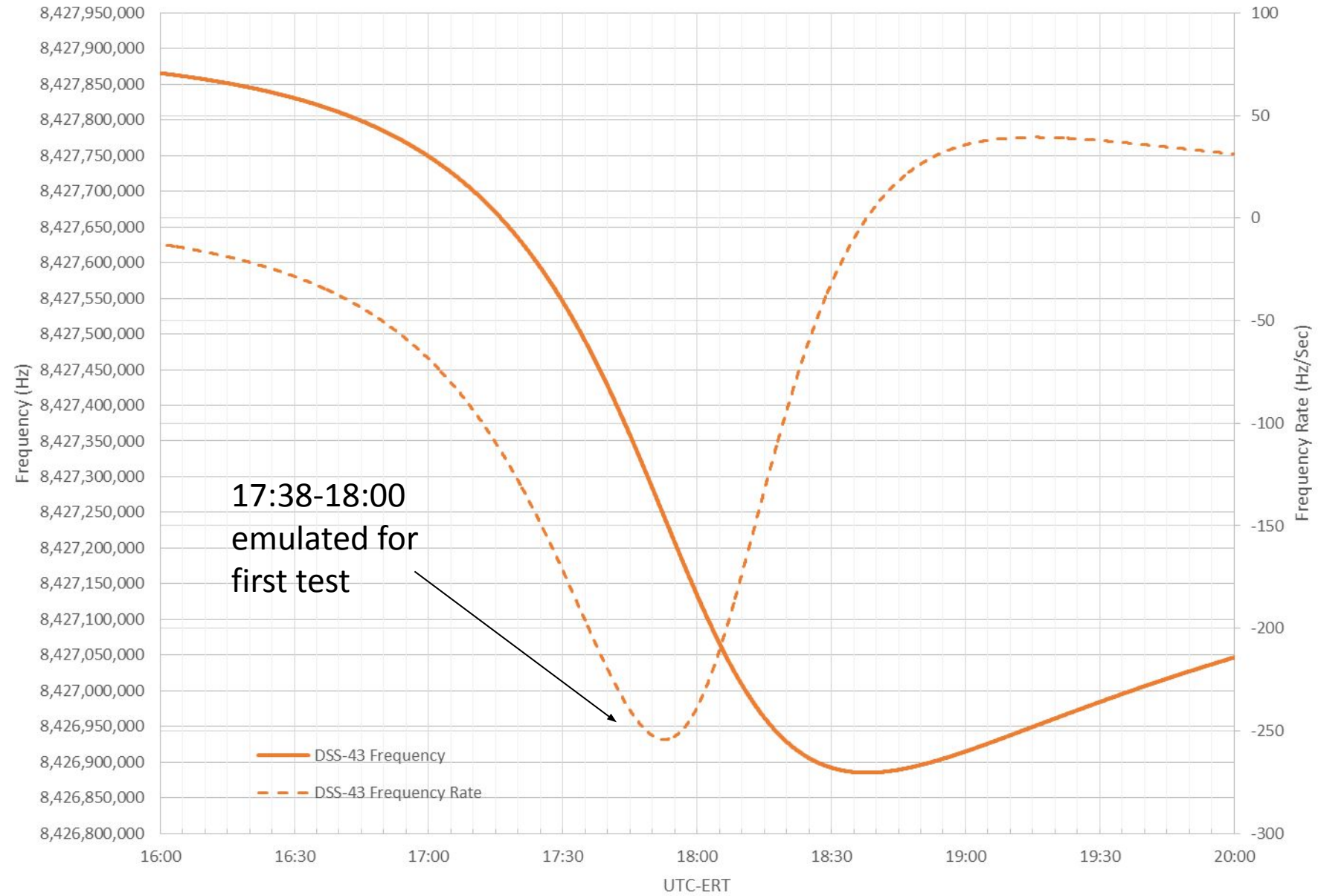
2017/135 18:02 Closest Approach (1-Way X-Band Downlink) Frequency & Rate
